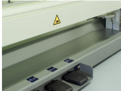
Foot pedal operation of the tie-bar and screen holder
